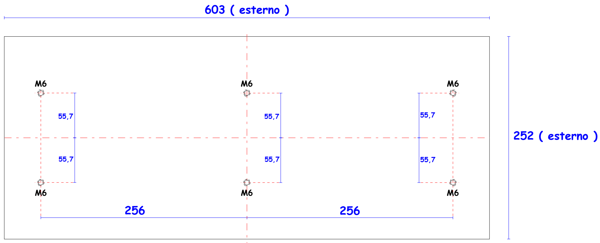
VISTA INFERIORE ( BOTTOM VIEW )
